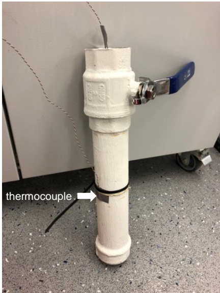
Figure 2 Pipe section sealed with RZ-Ecoseal
